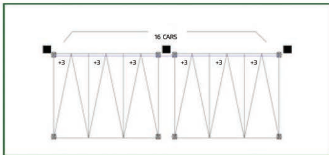
Good Column Placement, 16 Cars
